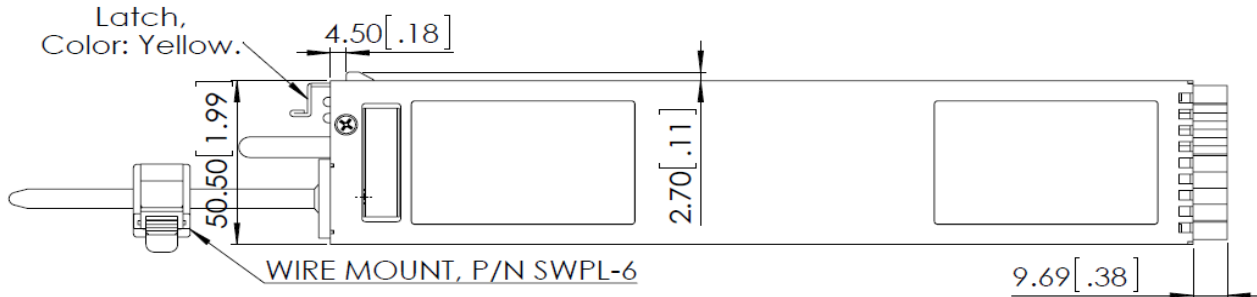
Bottom View
